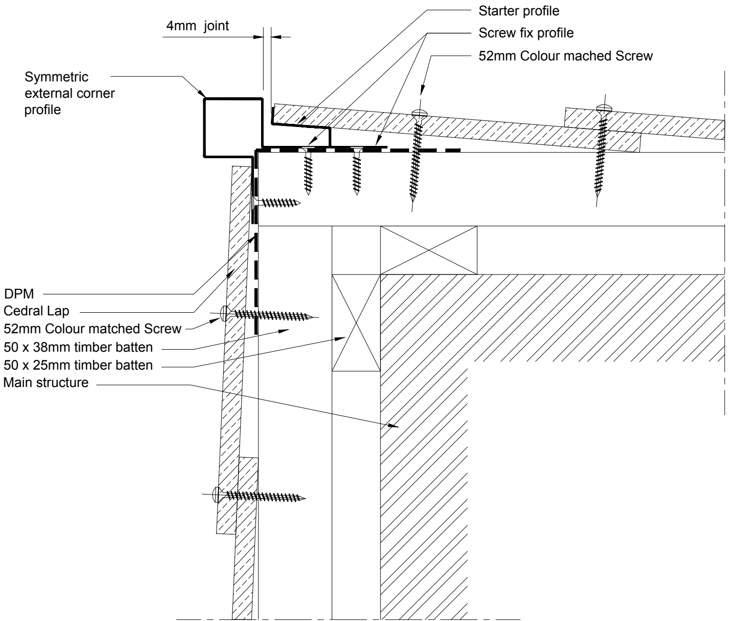
Plan on Profile 1:2
